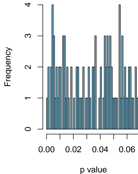
SVM-RFE
