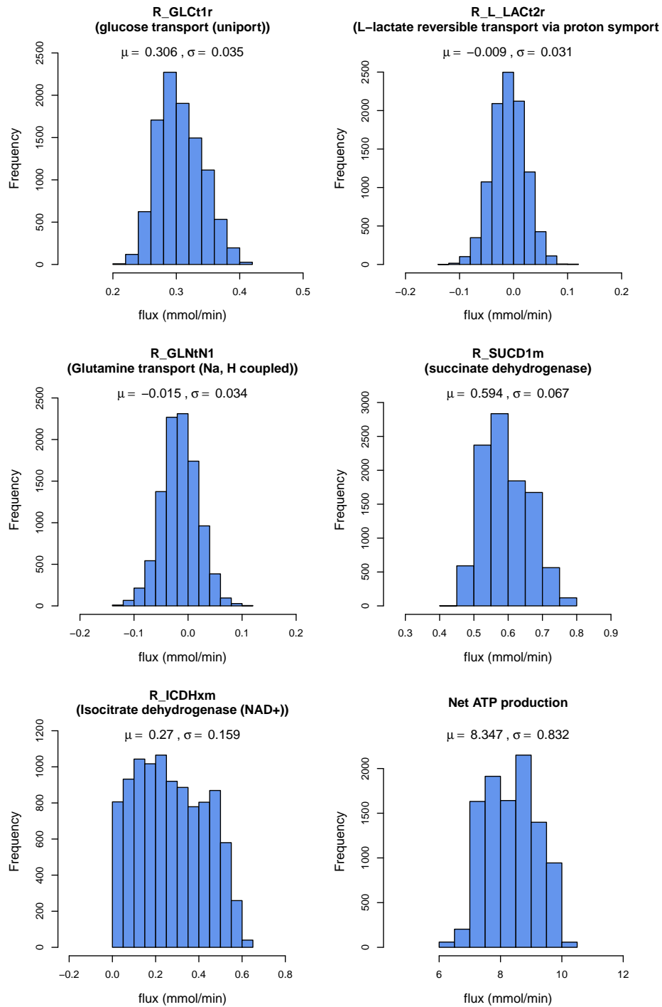
Figure 1: Posterior distributions of detected fluxes and the net ATP production rate after the sampling with Markov Chain Monte Carlo.
